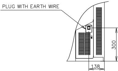
VIEW A(1/10)
